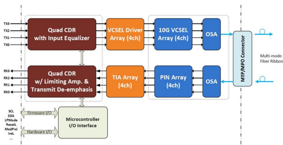
Figure1: Block Diagram
