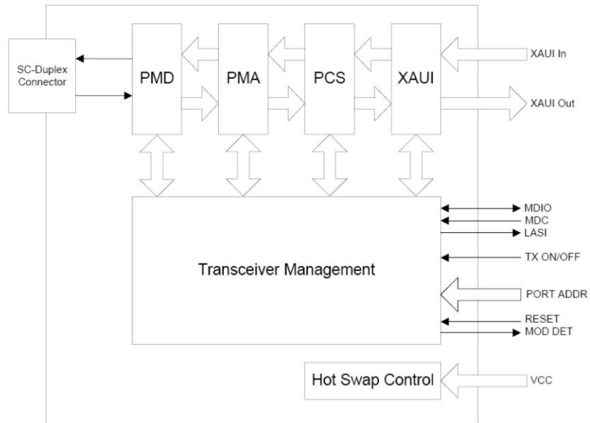
Figure1. Functional Diagram of Typical X2 Style Transceiver
