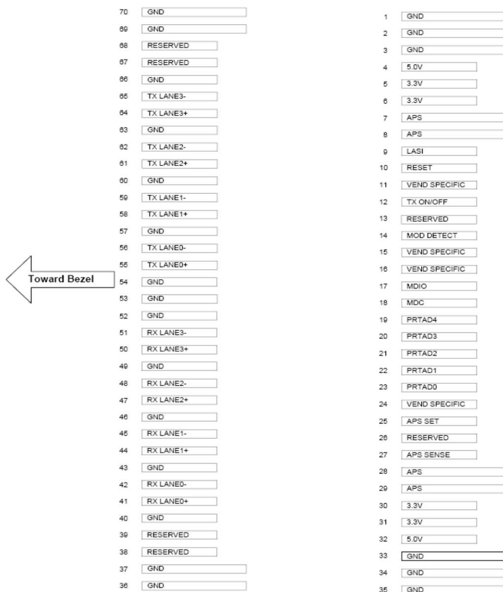
Figure2. Electrical Pin-out Details
