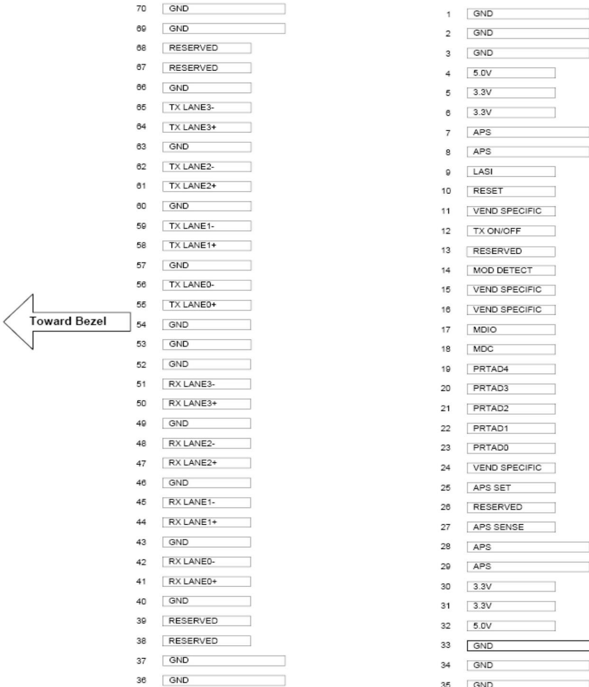
Figure2.Electrical Pin-out Details
