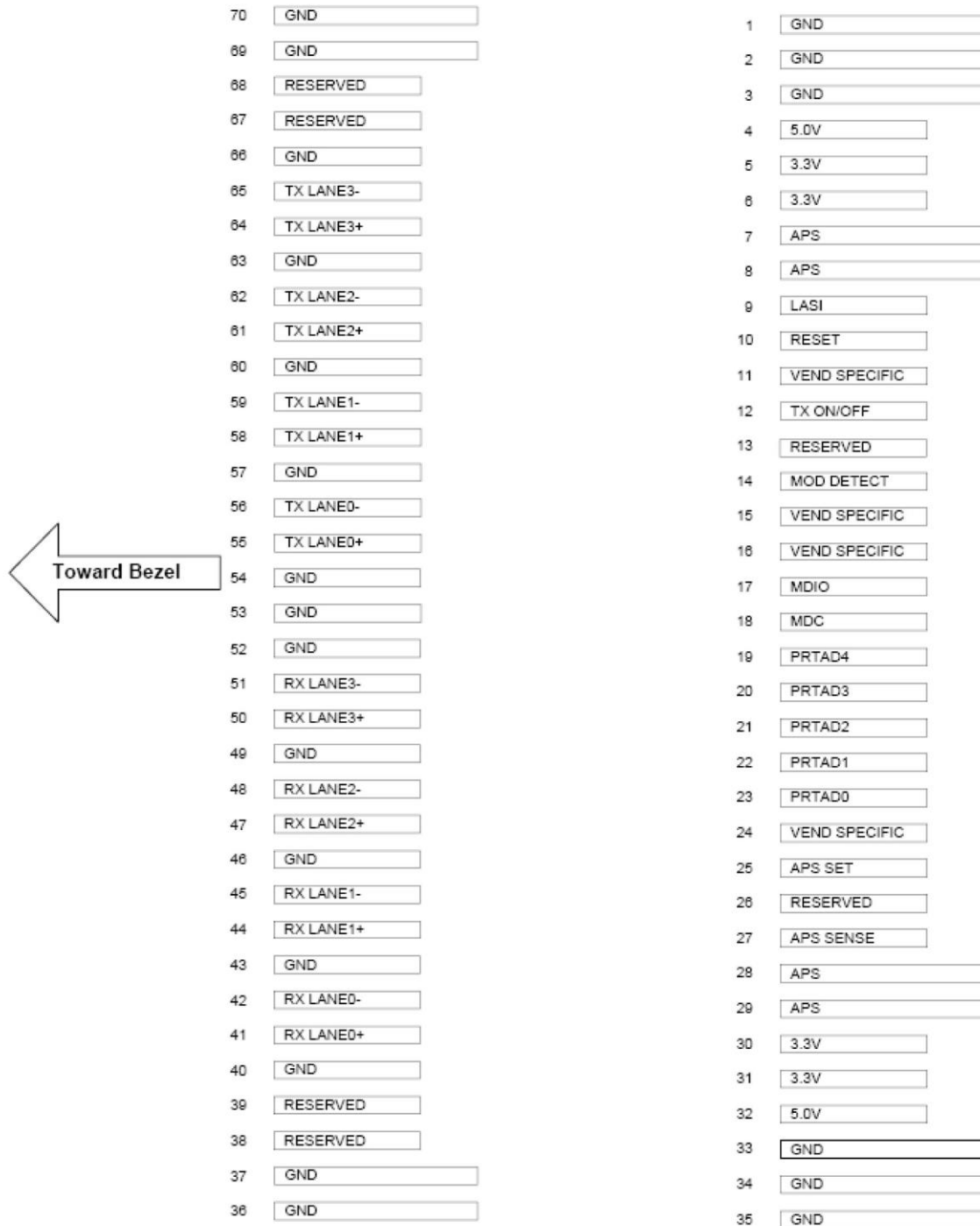
Figure2.Electrical Pin-out Details
