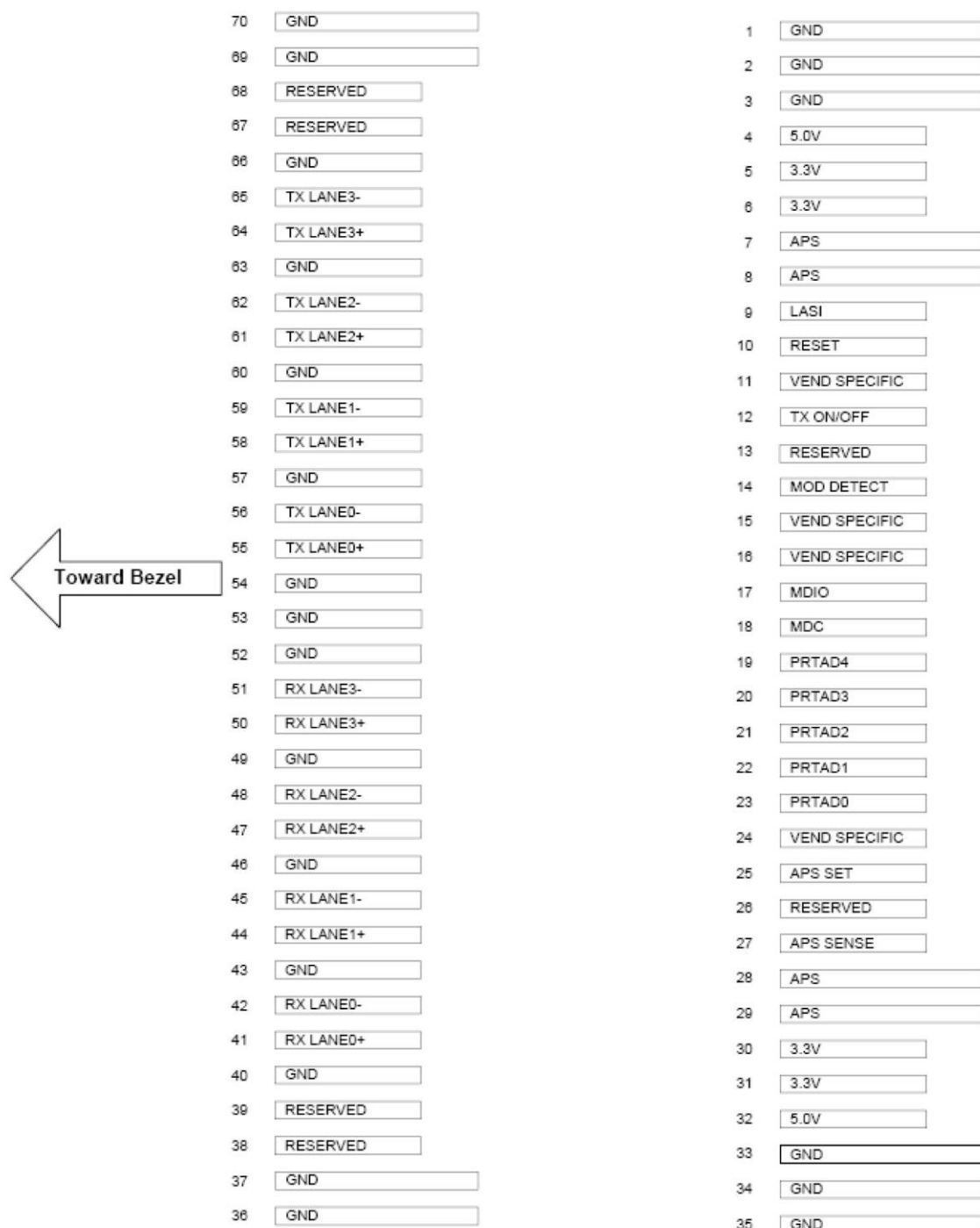
Figure2.Electrical Pin-out Details
