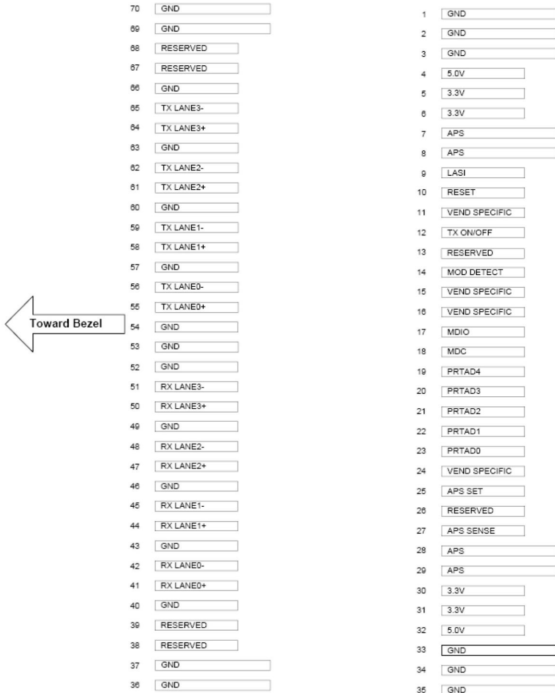
Figure2.Electrical Pin-out Details
