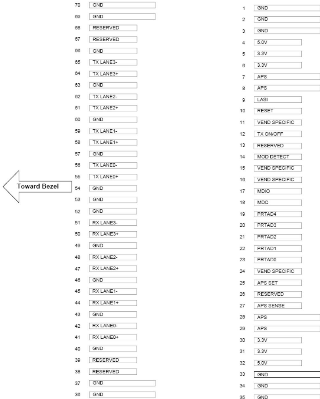
Figure2.Electrical Pin-out Details
